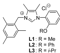
Figure 1. Ether-imidazolium chlorides.
